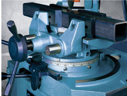
Miter Locking Device Standard Feature (not available for 275 PK or 275 PKPD models)
