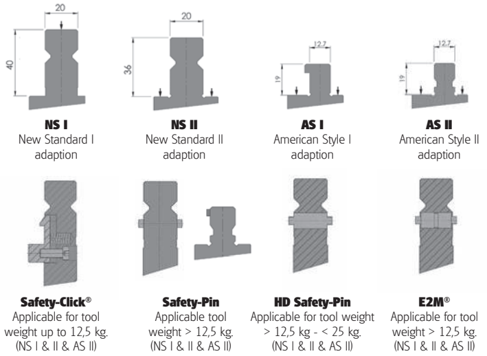
UPB (Universal Press Brake mounting to upper beam)*
